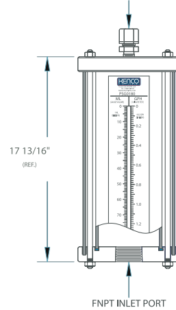
GAUGE WITH PVC END PLATES
