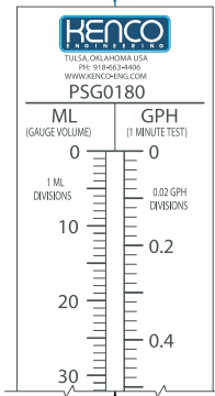
PSG0180 "GPH" SCALE CALIBRATION SCALE ILLUSTRATION
