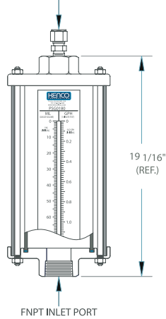
GAUGE WITH 316 S.S. END PLATES
